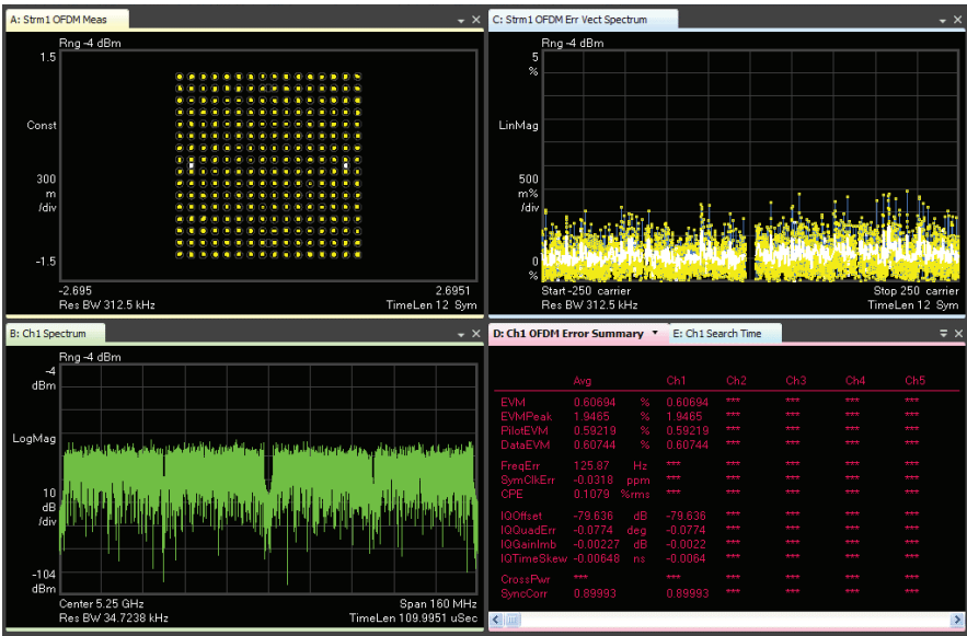
Figure 8-5. Modulation analysis of WLAN 802.11ac signal using Agilent 89600 VSA software
