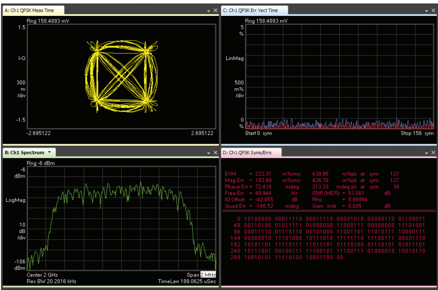
Figure 8-4. Modulation analysis of a QPSK signal measured with Agilent's 89600 VSA software
