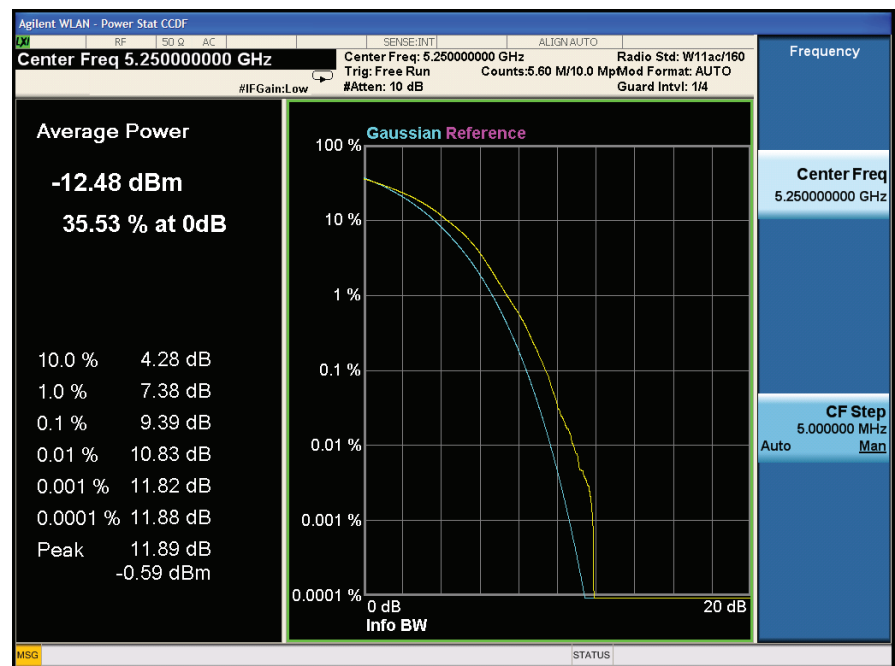
Figure 8-1. CCDF measurement
